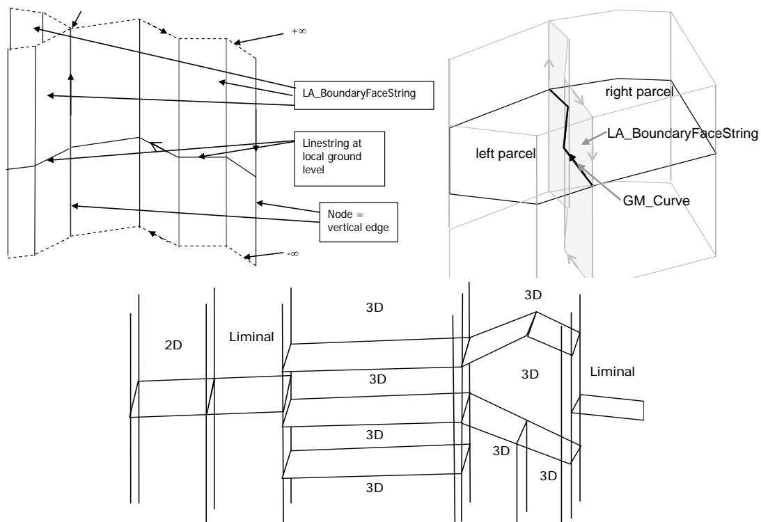
Figure 10. Top: Boundary face string concepts; Bottom: Side view showing the mixed use of boundary face strings and boundary faces to define both bounded and unbounded 3D volumes (from ISO/TC211, 2012)
