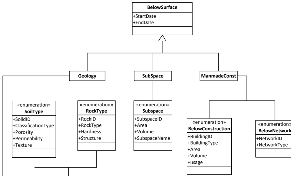
Figure 6. Below Surface classes and data enumerations
