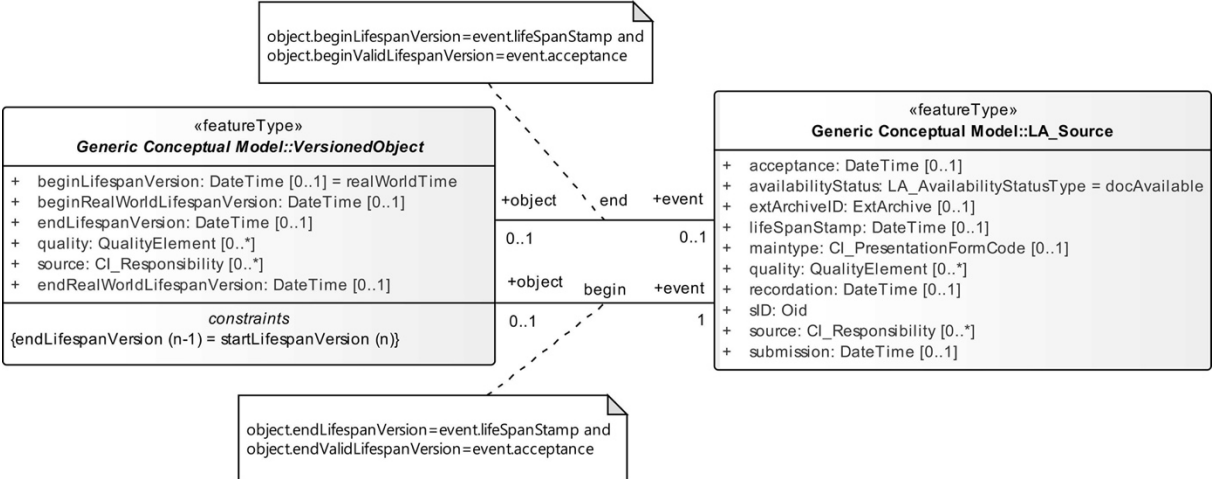
Figure 4. Versioned Object in LADM II (Source: ISO 19152-1 Generic conceptual model https://www.iso.org/standard/81263.html )
