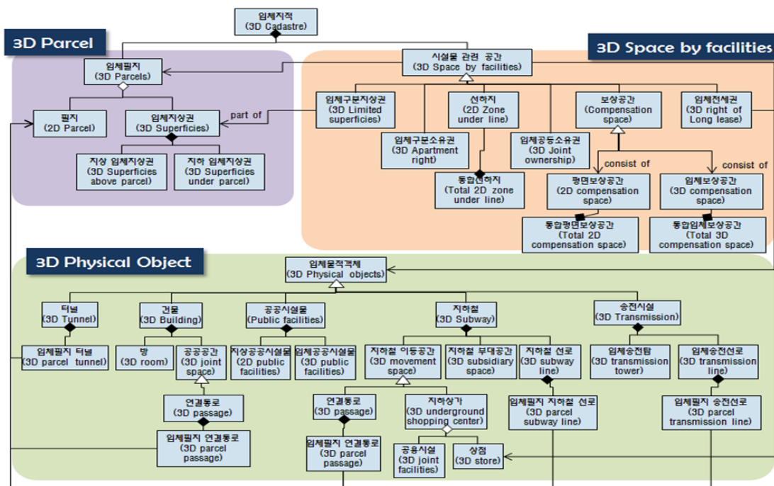
Figure 2. UML diagram of the integrated object model
