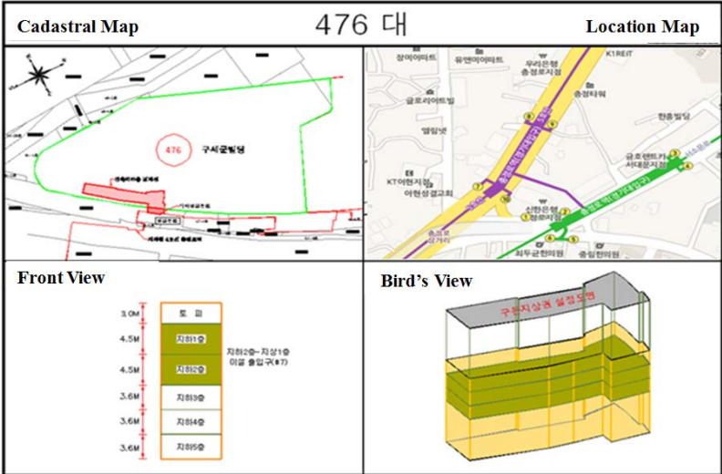
Figure 4. An example of suggested 3D cadastral drawing
