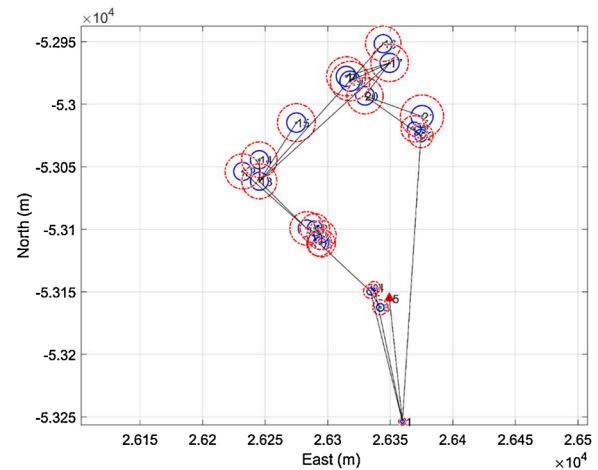
Fig. 3. Illustration of uncertainties: Blue circles show the standard deviations, while red circles represent the uncertainties in the confidence level of 95%. (For interpretation of the references to colour in this figure legend, the reader is referred to the web version of this article).
