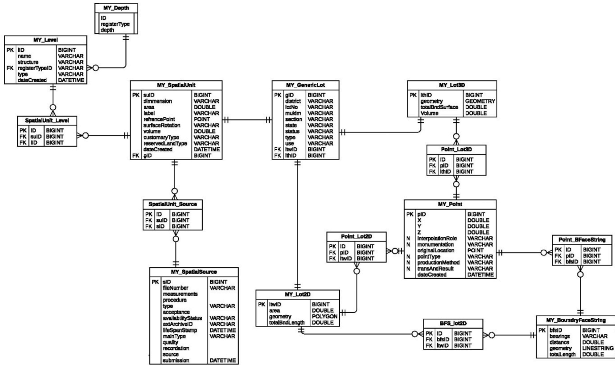
Fig. 5. Spatial and survey elements in 3D-NDADB.
