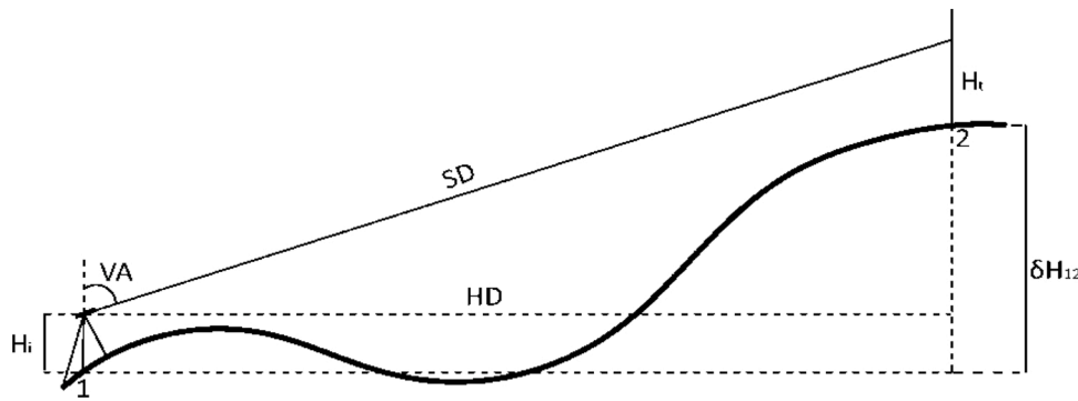
Fig. 1. A schematic of Trigonometry.
