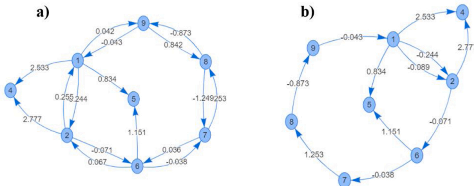
Fig. 4. a) A height network including 2 independent sets of measurements on each edge of the major loop. b) A height network without independent measurements on each edge (the independent set of observation between node 1-2 is only added to show the values).
