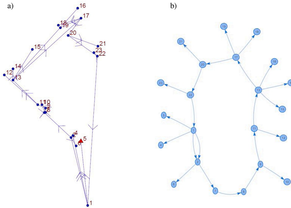
Fig. 2. a) A height network, b) Graph of loops in the height network.
