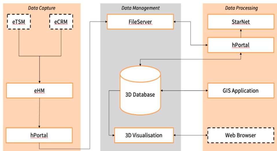
Fig. 7. Architecture of prototype system.
