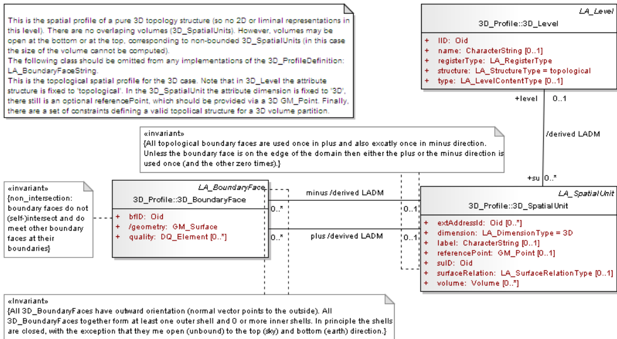
Figure 1a. Data model in LADM. 3D Topology spatial profile, from Annex E (ISO/DIS 19152, 2010)
