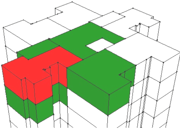
Figure 19. Topological query
