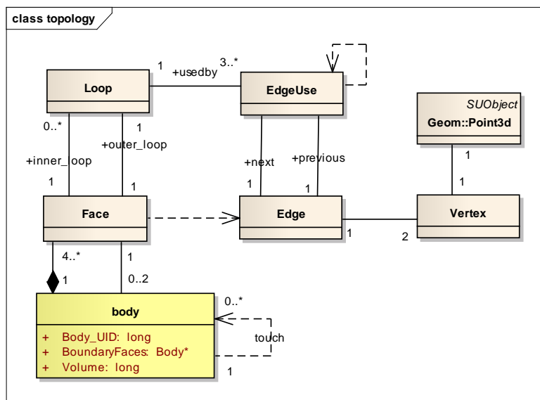
Figure 4. Data model in SketchUp
