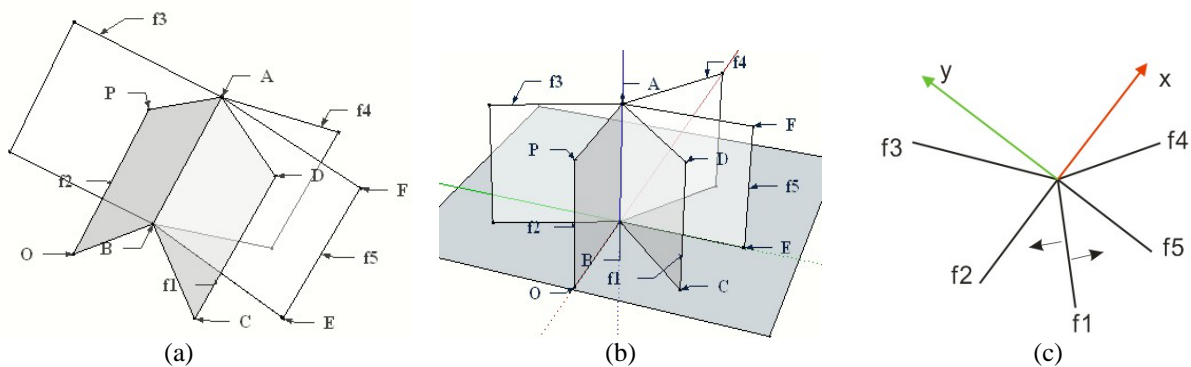
Figure 8. Face-sorting based on shared edge
