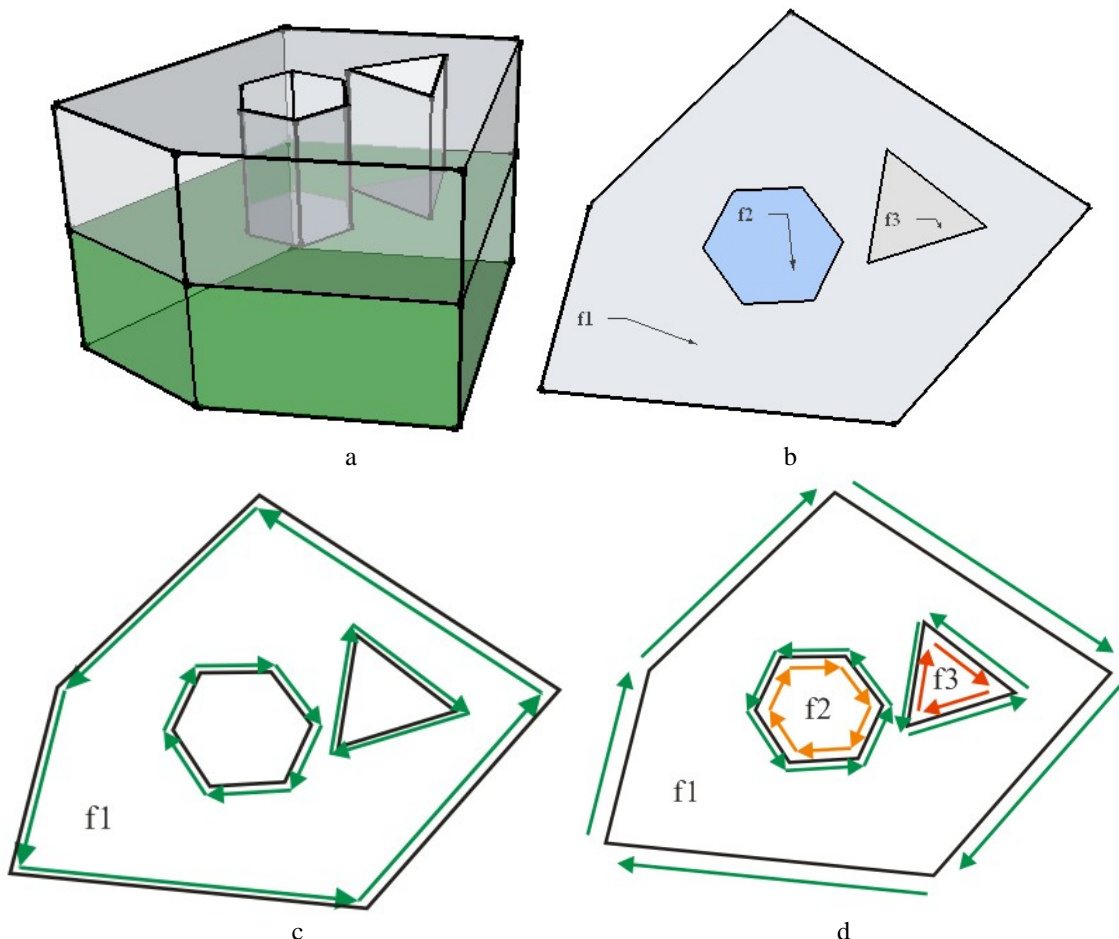
Figure 6. Face with inner holes and its different roles in the different bodies
