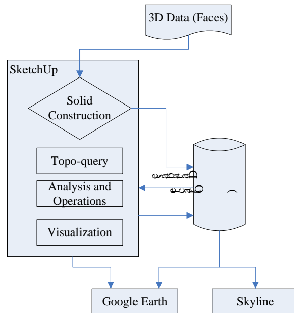
Figure 14. Framework of the prototype
