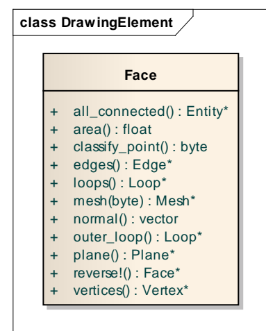
Figure 5. Functions in class Face
