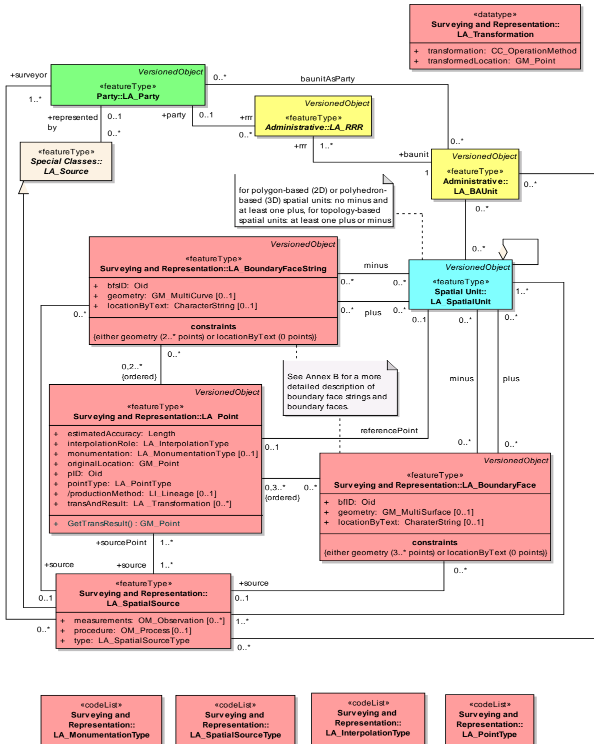
Figure 1b. Data model in LADM, overview spatial representation (ISO/DIS 19152, 2010)
