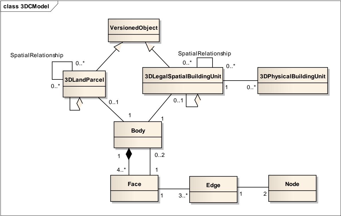
Figure 2. Data model in prototype system
