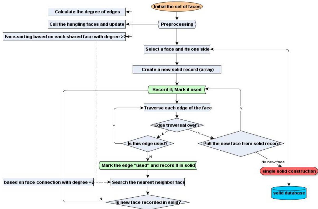
Figure 10. Workflow of the automatic construction of the valid solid based on shared edge
