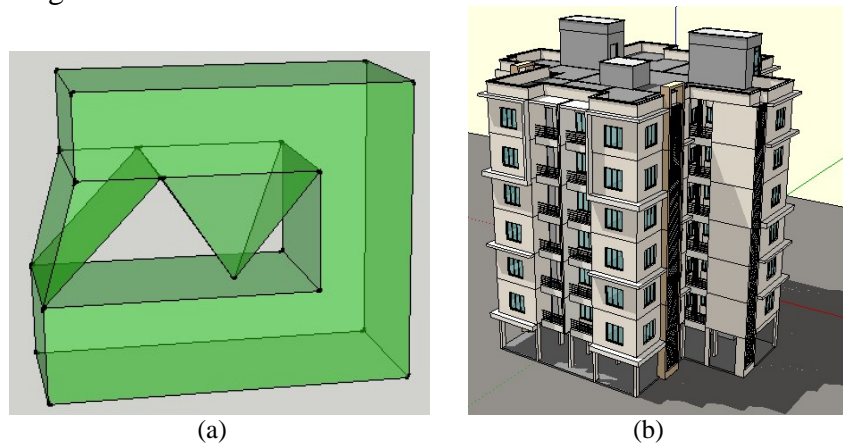
Figure 13. Non-manifold conditions: a) non-manifold valid solid; b) body collection
