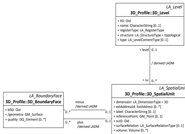
Figure 2. 3D topology based on LADM (after ISO 19152: 2012)
