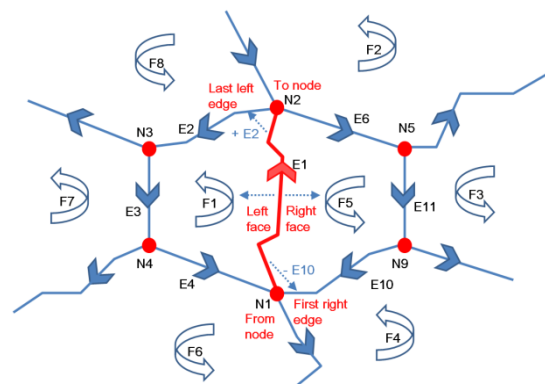
Figure 1. 2D topology model as used in the Malaysian country profile
