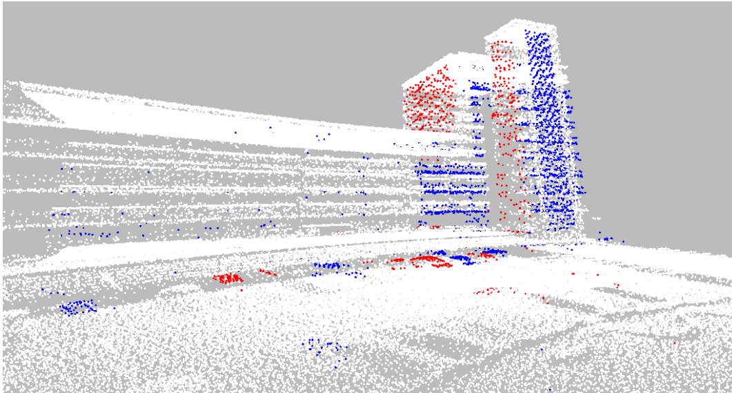
Figure 6. Detected changes due to differences in the viewing angle
