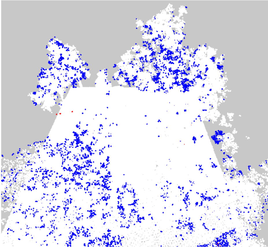
Figure 4. Effect of vegetation growth on change detection
