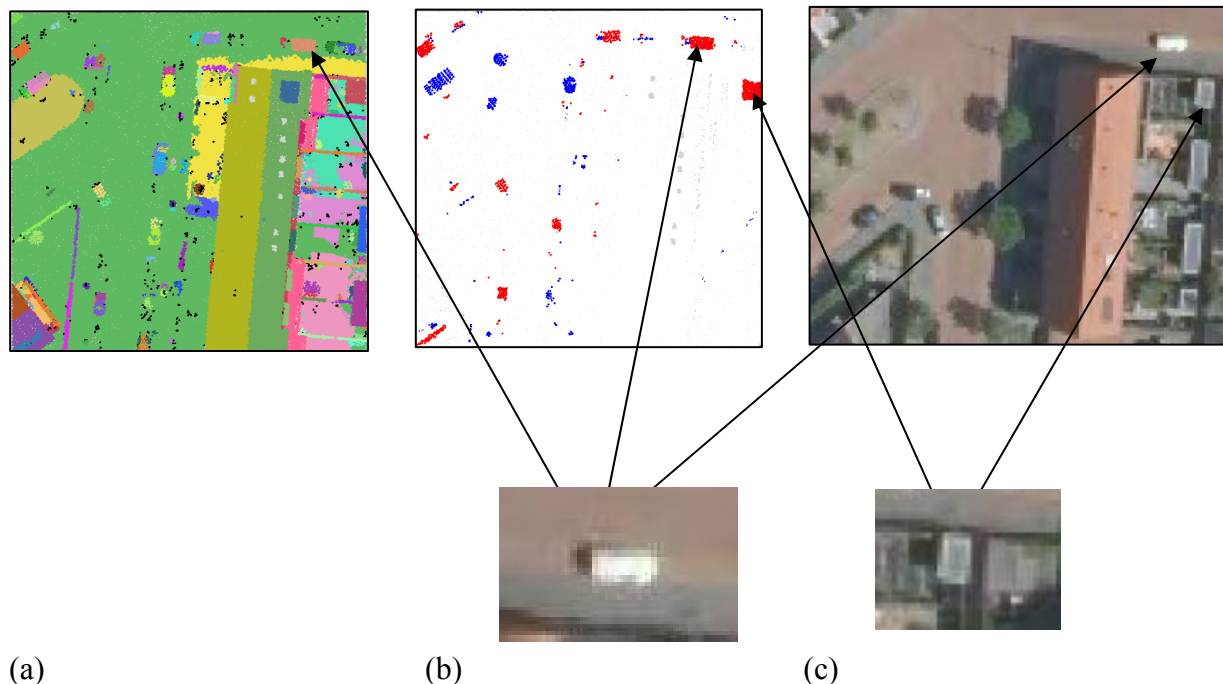
Figure 2. Detected changes while overlaying ALS point clouds from epoch1 and epoch 2
