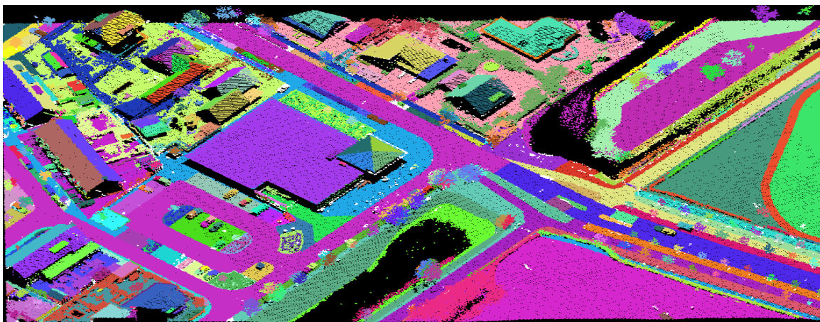
Figure 8. Result of map based segmentation for multi-land-cover landscape. Source: (Wang, 2016)
