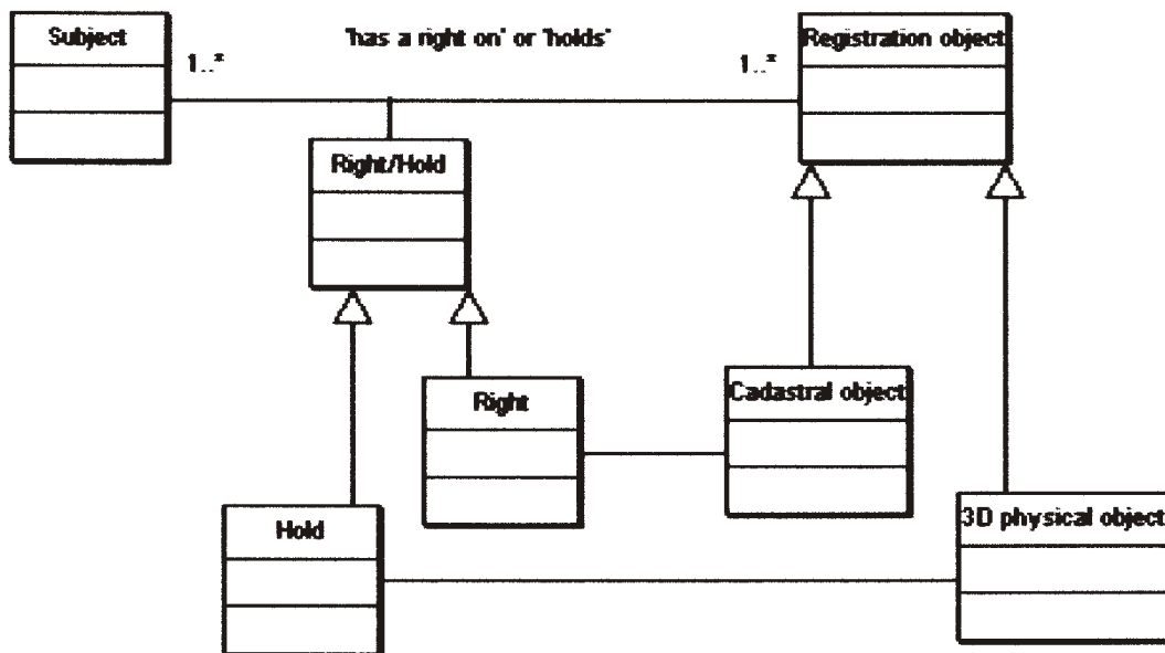
Figure 11: UML class diagram of 3D physical objects
