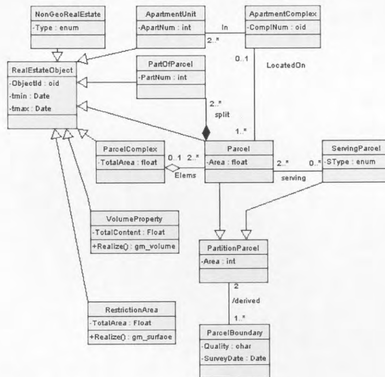
Figure 2. The RealEstateObject package refined ('blue' part)
