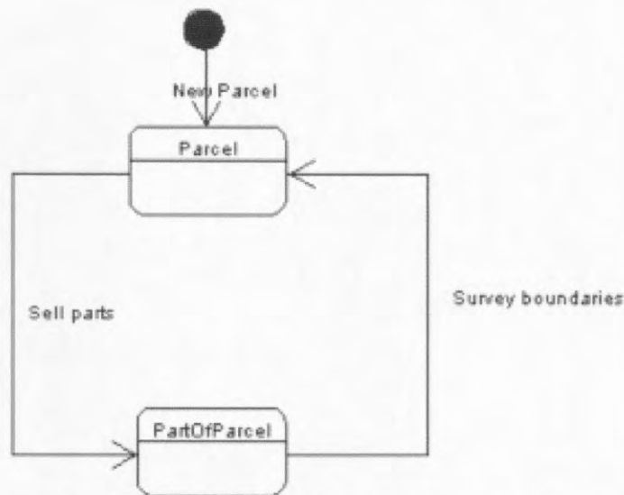
Figure 6: State diagram of splitting a Parcel. If a part of a parcel is sold, the parcel is split into several PartOfParcels, which become regular parcels again only when their boundary is surveyed.
