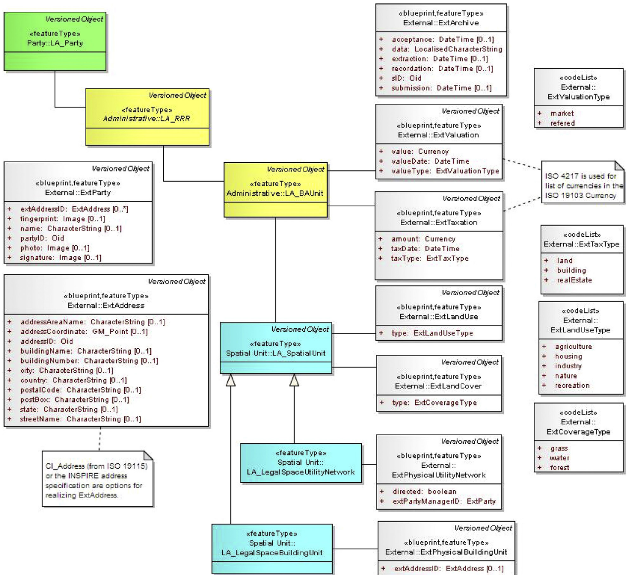
Fig. 5. External classes.
