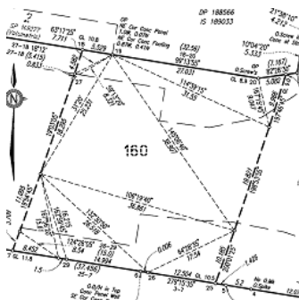
(a) 3D Footprint on cadastral plan
