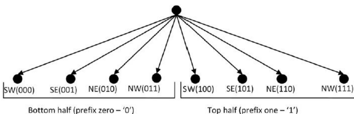
Figure 10. 3D space decomposition (Schön et al., 2013)
