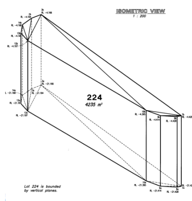
(b) Isometric view on cadastral plan
