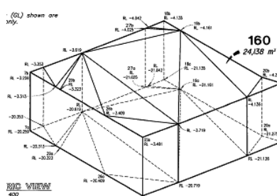
(b) Isometric view on cadastral plan
