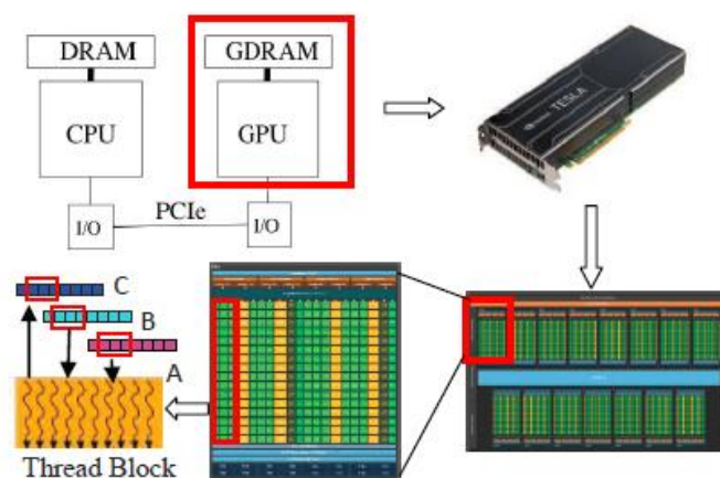
Figure 22. Illustration of GPU hardware Architecture (according to (Zhang et al., 2015c))
