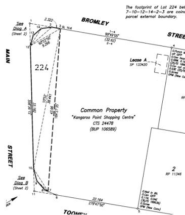
(a) 3D Footprint on cadastral plan
