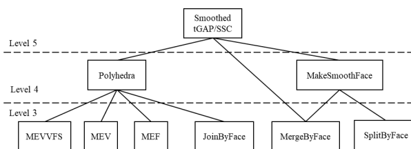
Figure 4. Construction operators are organized in layers:
